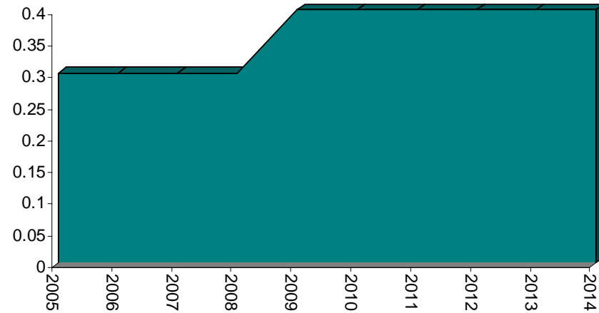
Ferromanganese production capacity (mtpa)
